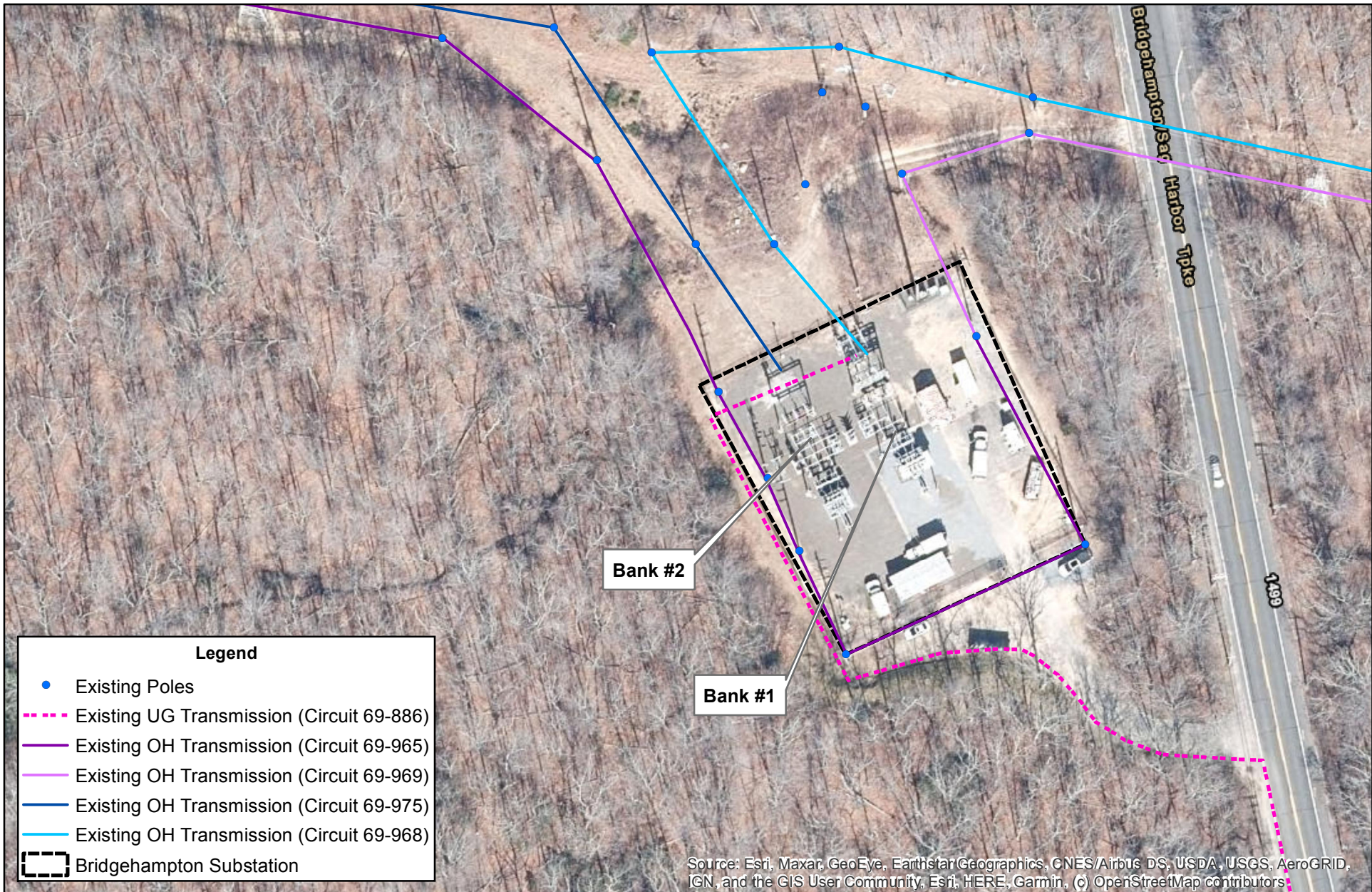
FIGURE 2 BRIDGEHAMPTON SUBSTATION NEW BANK AND HALF LINE UP SWITCHGEAR EXISTING TRANSMISSION CIRCUITS MAP
